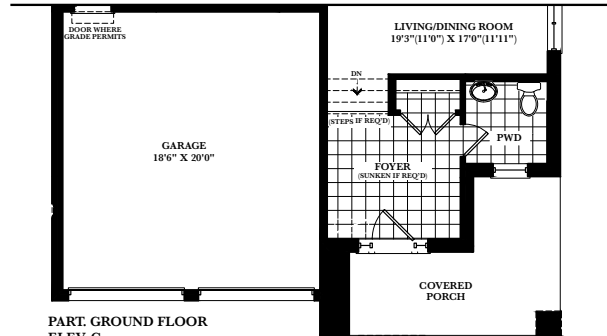
PART. GROUND FLOOR ELEV. C
