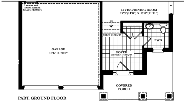
PART. GROUND FLOOR ELEV. B
