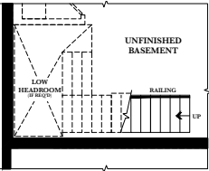
OPT. PART. BASEMENT ELEV. A, B & C SERVICE STAIRS
