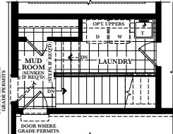
OPT. PART. GROUND FLOOR ELEV. A, B & C SERVICE STAIRS
