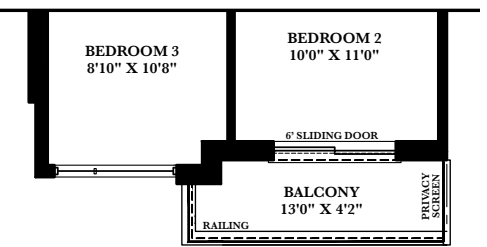
PART: THIRD FLOOR ELEV. C
