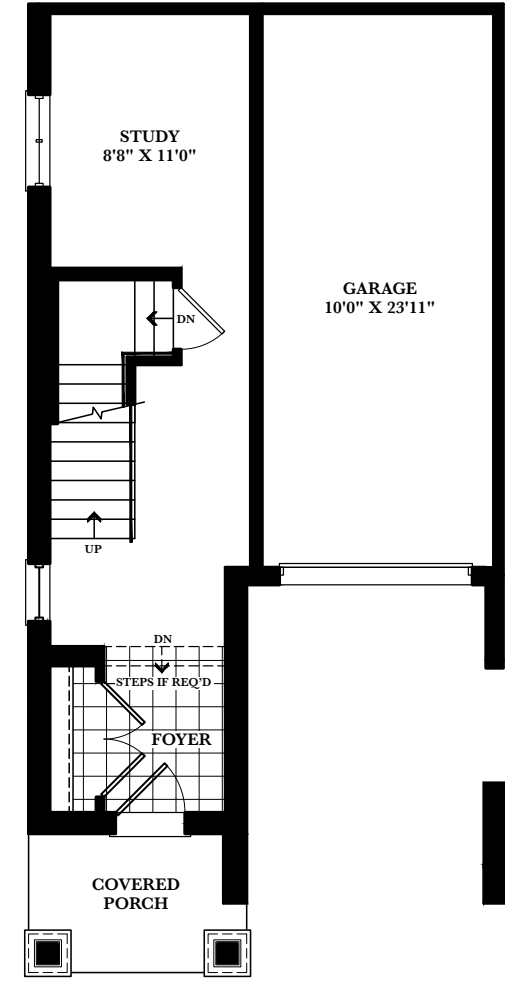
GROUND FLOOR ELEV. B
