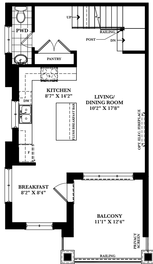
SECOND FLOOR ELEV. B
