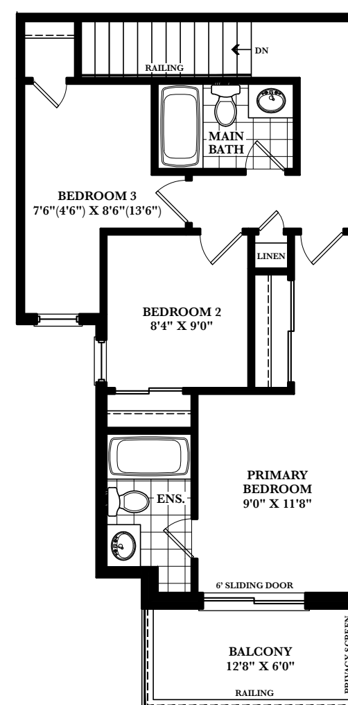
OPT. THIRD FLOOR ELEV. B & C
