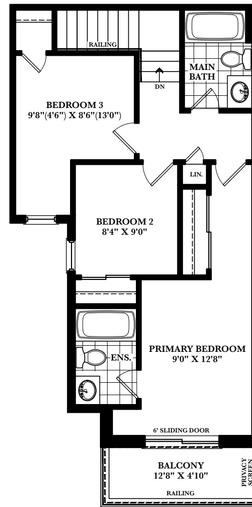
OPT. THIRD FLOOR ELEV. B & C
