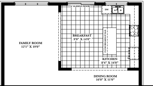
PART ALT. GROUND FLOOR ELEV. A, B & C
