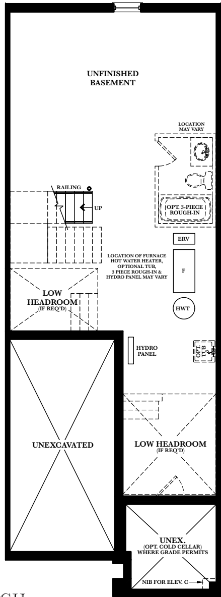
BASEMENT ELEV. B & C
