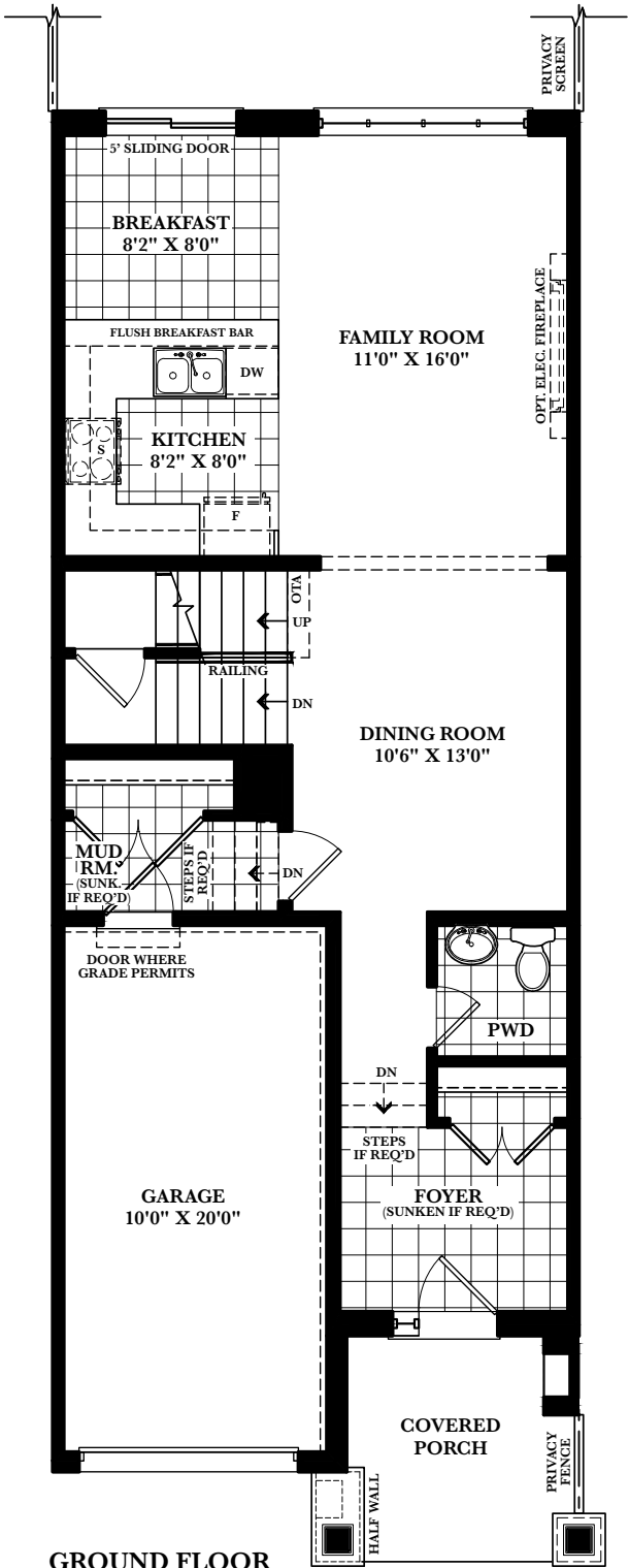
GROUND FLOOR ELEV. B
