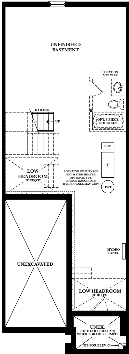
BASEMENT ELEV. B & C
