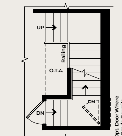
ALT. ENCLOSED STAIR LAYOUT
