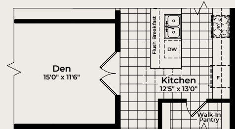
PART. GROUND FLOOR W/ Opt. Den Elev. A, B & C
