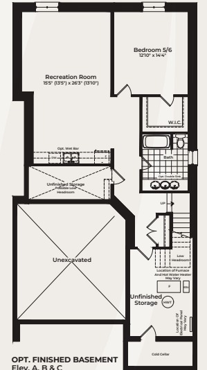
OPT. FINISHED BASEMENT Elev. A, B & C
