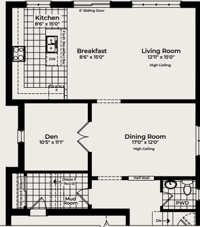
PART. ALT. GROUND FLOOR W/ DEN Elev. A, B & C
