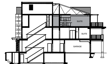
TYPICAL CROSS SECTION BUILDING 1, 2, 3 & 4
