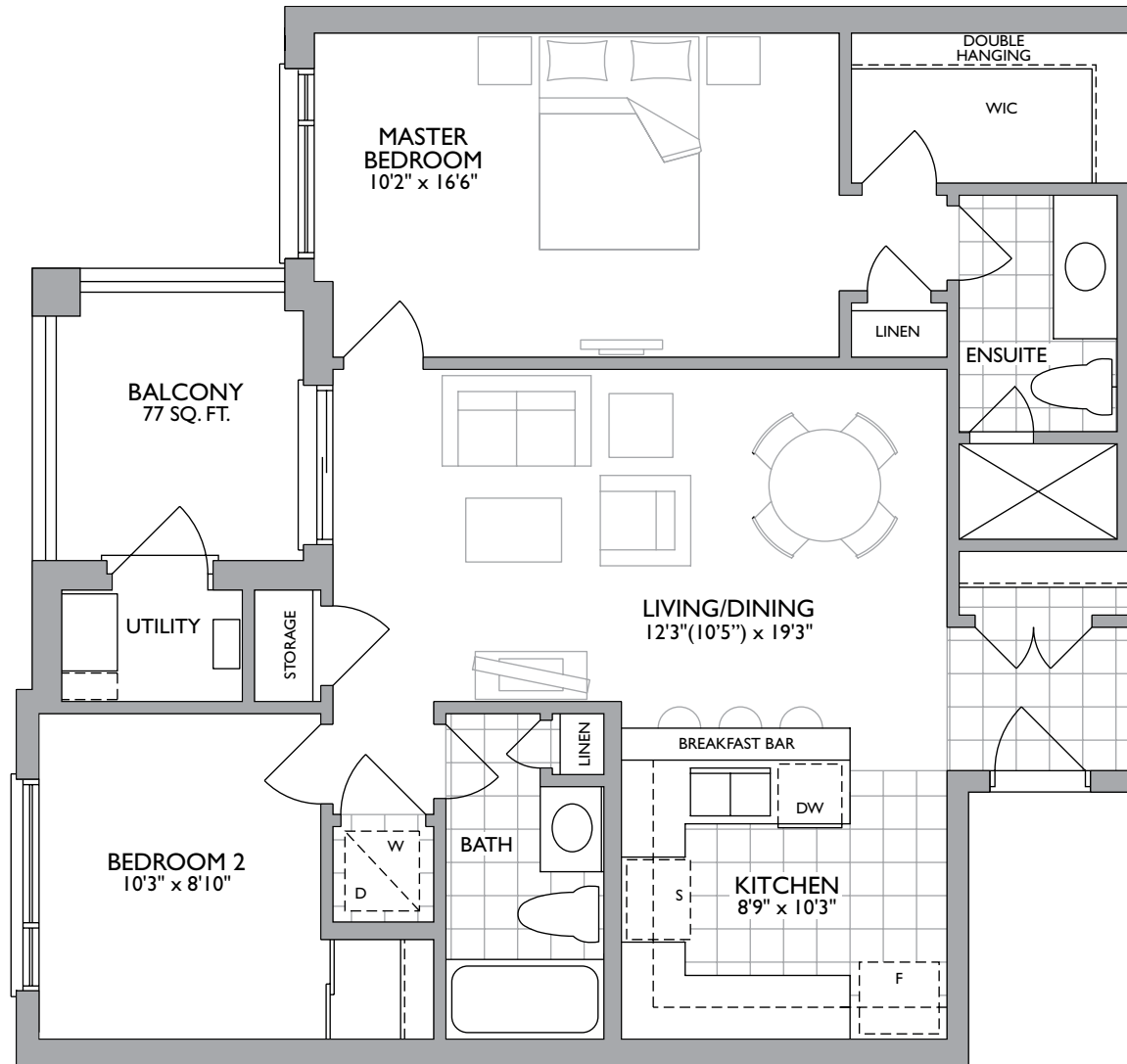
THIRD FLOOR ELEVATION A SUITE 303/304
