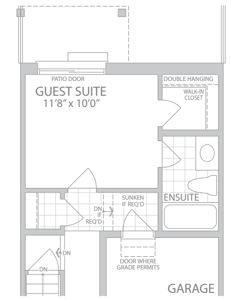
OPT. GROUND FLOOR ELEV. A GUEST SUITE IN LIEU OF FAMILY ROOM
