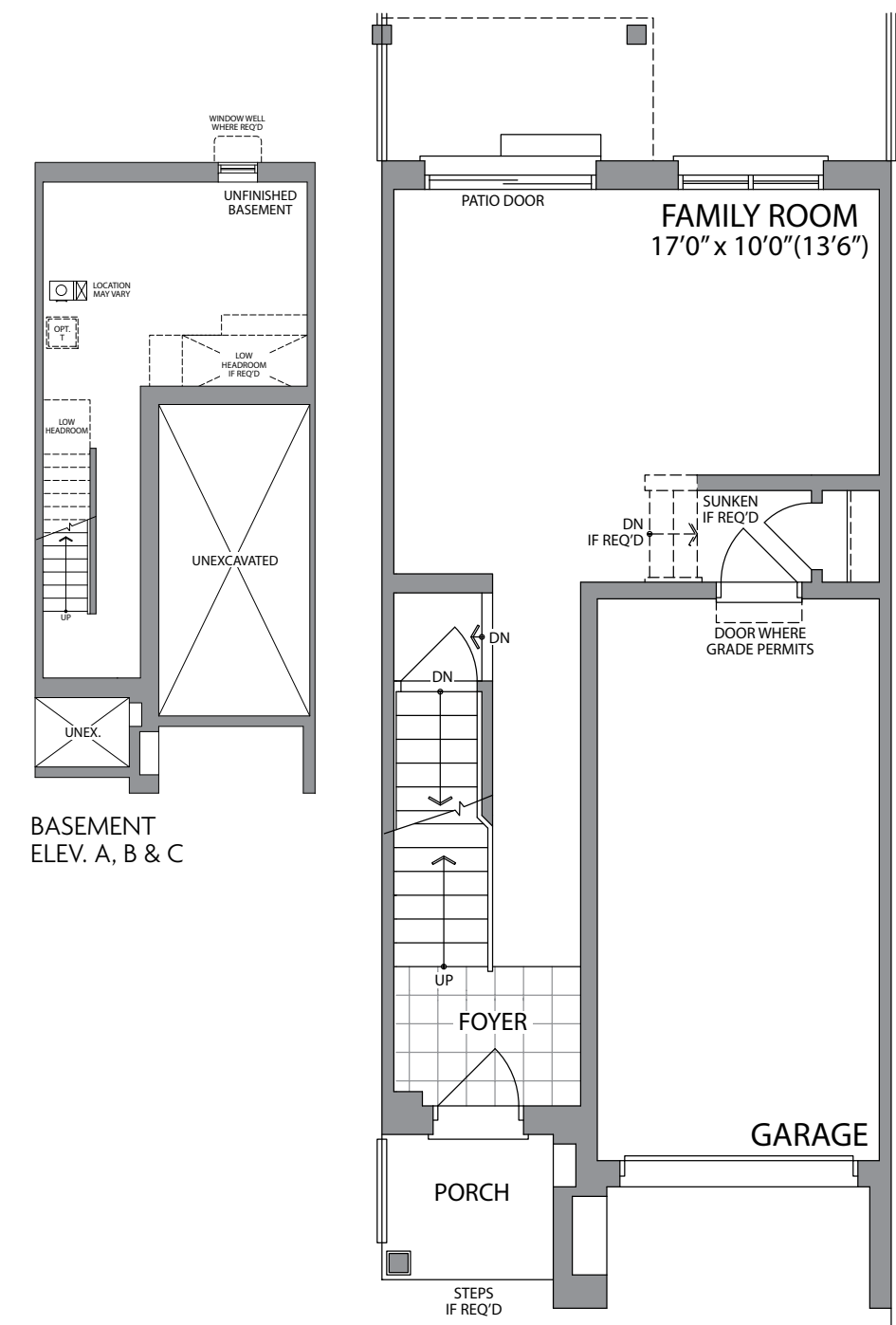
GROUND FLOOR ELEV. A, B & C
