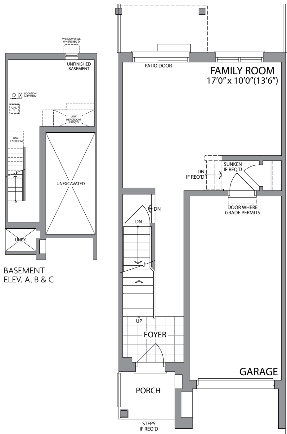
GROUND FLOOR ELEV. A, B & C
