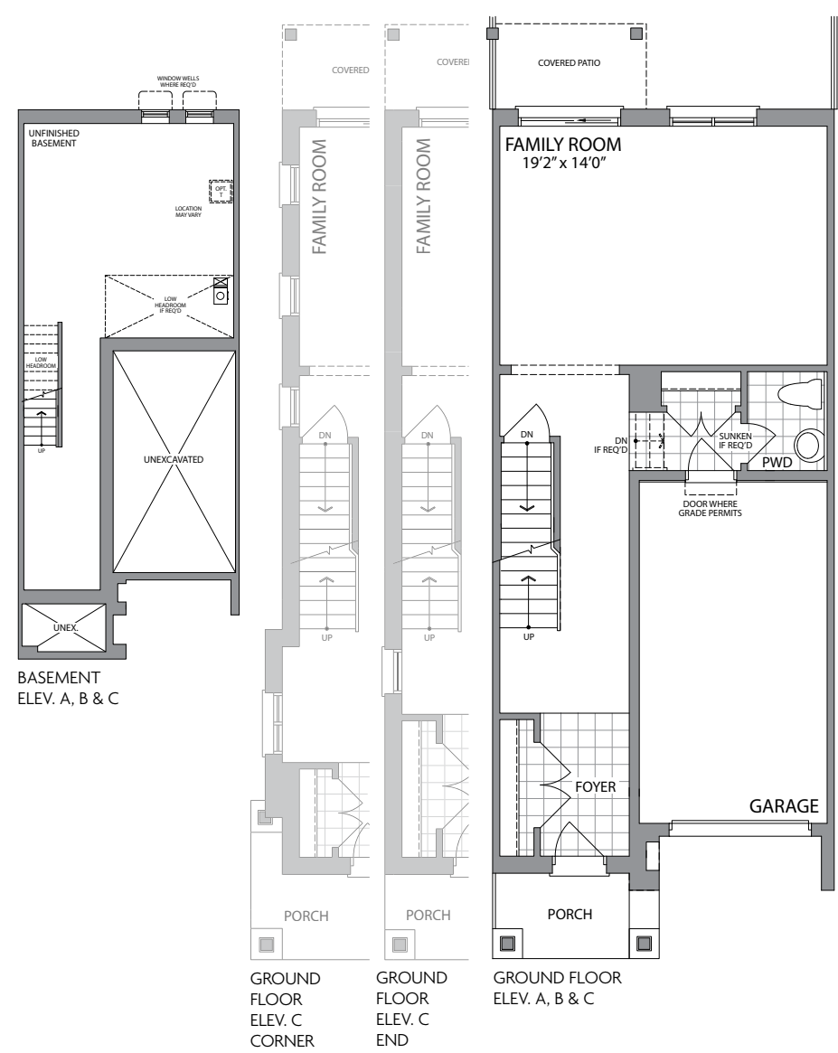
MAIN FLOOR ELEV. C CORNER
