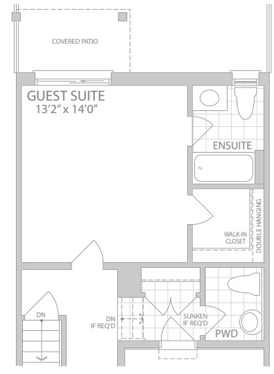
OPT. GROUND FLOOR ELEV. A, B & C GUEST SUITE W/ENSUITE
