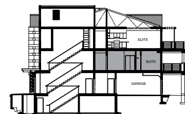
TYPICAL CROSS SECTION BUILDING 1, 2, 3 & 4
